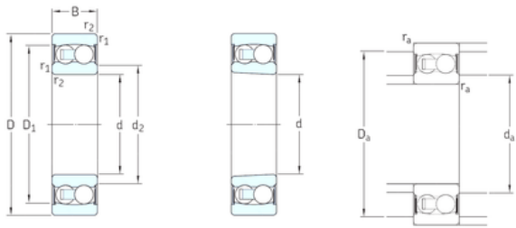
Cylindrical bore
